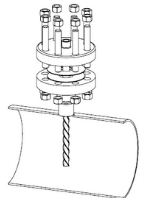
RF flange helical solid machined thermowell
