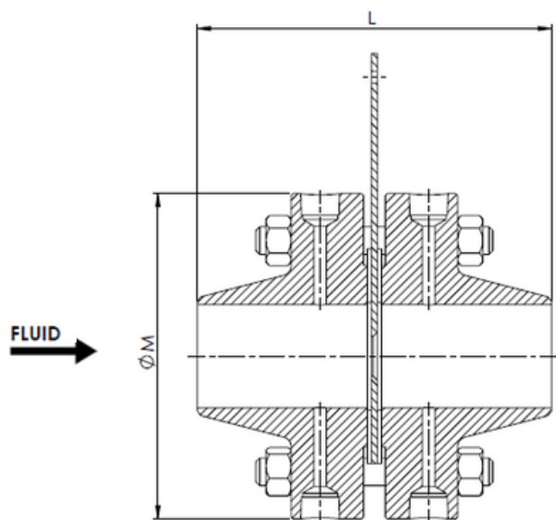
RF flange tap flowmeter
