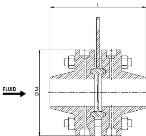
RTJ-M flange tap flowmeter
