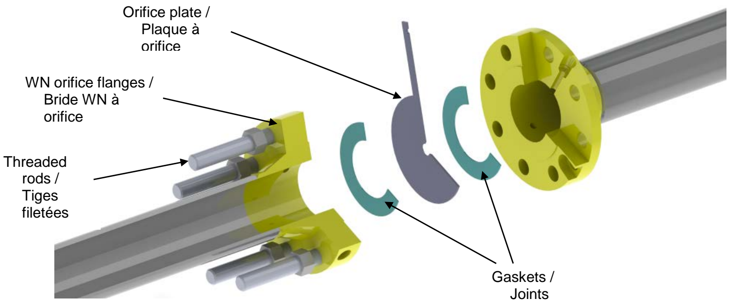
Fig 4 : Assembly on the orifice plate between flanges Fig 4 : Montage de la plaque à orifice entre brides
